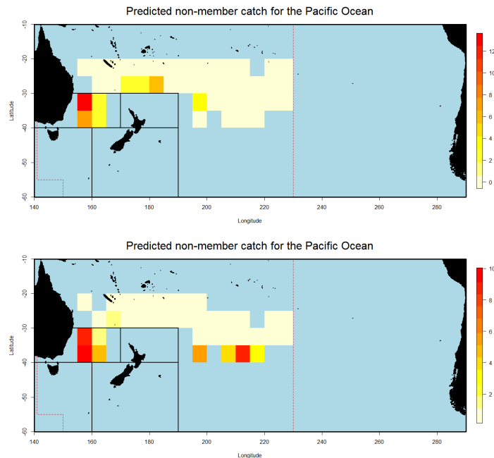
Figure 16. Map of average annual predicted non-Member catch in the Pacific Ocean, in tonnes, from the GLM (top) and random forest (bottom) analyses. Results average two alternate assumptions concerning catchability of the non-Member fleet (i.e. assumed Japanese or Taiwanese catchability) and use the adjusted CCSBT catch rate data used to parameterise the model.
