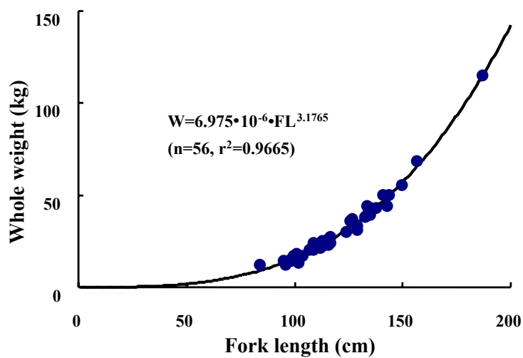
Fig. 2. Weight-length relation of southern bluefin tuna caught in the central Indian Ocean
