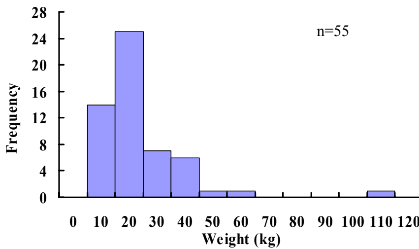
Fig. 4. Weight-frequency distributions of southern bluefin tuna caught in the central Indian Ocean
