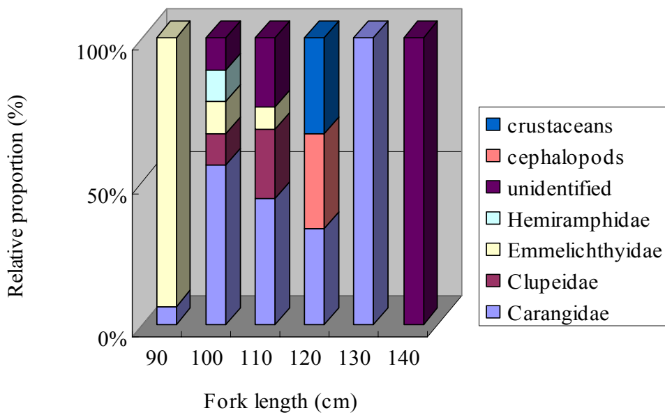
Fig. 5. Relative proportions of the main preys of southern bluefin tuna caught in the central Indian Ocean.
