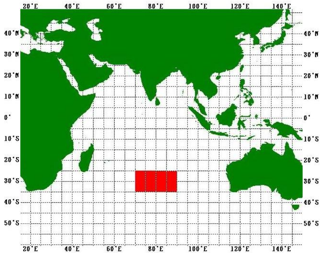
Fig. 1. Sampling area of southern bluefin tuna caught by Taiwanese longliners in the central Indian Ocean.
