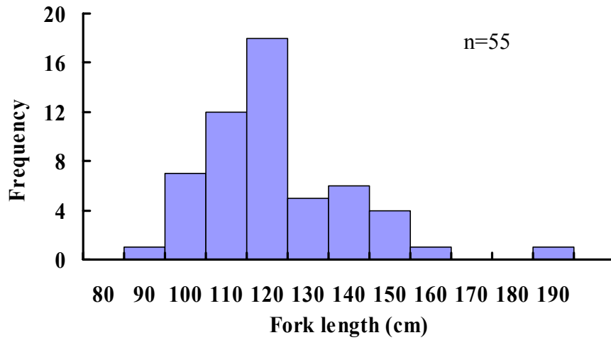
Fig. 3. Length-frequency distributions of southern bluefin tuna caught in the central Indian Ocean
