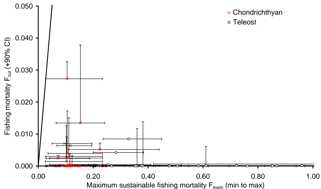
Figure 7-2. Comparison of estimated fishing mortality in the recent years (2004-2007) F_{cur} and the reference fishing mortality corresponding to the maximum sustainable mortality for fish species caught in the Western Tuna and Billfish Fishery . The diagonal line is where F_{cur} = F_{msm} .
