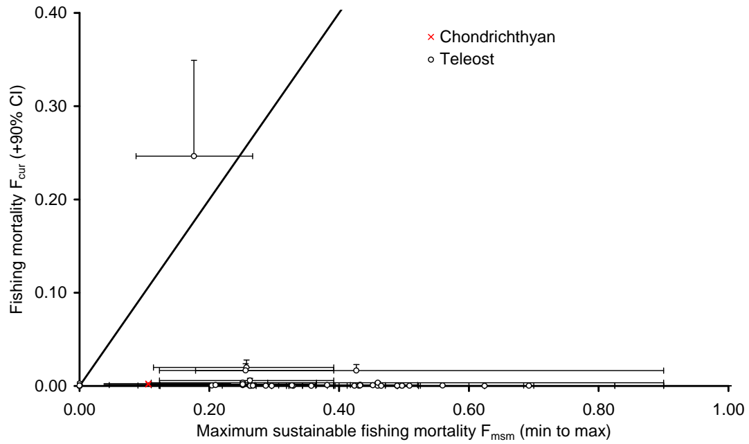
Figure 8-9. Comparison of estimated fishing mortality in the recent years (2004-2007) F_{cur} and the reference fishing mortality corresponding to the maximum sustainable mortality for fish species caught in the Macquarie Island Demersal Trawl Sub-fishery . The diagonal line is where F_{cur} = F_{msm} .
