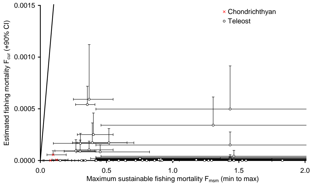
Figure 4-5. Comparison of estimated cumulative fishing mortality in the recent years (2004-2007) F_{cur} and the reference fishing mortality corresponding to the maximum sustainable mortality for fish species caught in the Small Pelagic Fishery . The diagonal line is where F_{cur} = F_{msm} .
