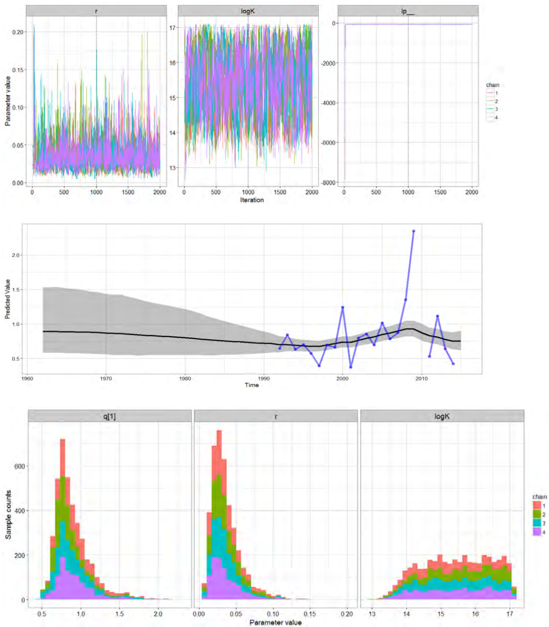
Figure 20. Top: Trace outputs from the MCMC model fit showing estimates of r and \log(K) alongside the log-posterior ( lp_{\_} ). Middle: Derived fit to the CPUE index. Bottom: Stacked histograms of MCMC samples, representing the posterior distributions of q , r and \log(K) .
