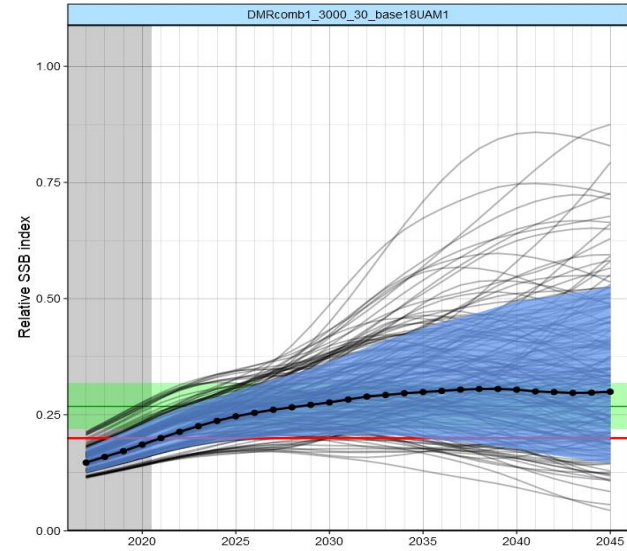
Figure 2e. Worm plots for TAC and TRO (reported as “Relative SSB index”) for DMRCOMB1 , when tuned to 30% of TRO_0 in the year 2035, for the RC (base18). The blue shadings represent 95% probability envelopes, and the bold line with dots shows the medians. In the TRO plots, the red line is the SSB level corresponding to the interim rebuilding target (0.20 SSB_0 ) of the Extended Commission, and the green band represents the 80% confidence interval for the maximum sustainable yield (MSY), with the median as the horizontal green line. The TAC axis upper bound is at the maximum TAC of 28 000 mt which the CMP allows.
