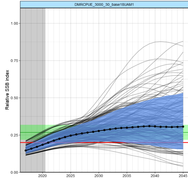
Figure 2a. Worm plots for TAC and TRO (reported as “Relative SSB index”) for DMRCPUE , when tuned to 30% of TRO_0 in the year 2035, for the RC (base18). The blue shadings represent 95% probability envelopes, and the bold line with dots shows the medians. In the TRO plots, the red line is the SSB level corresponding to the interim rebuilding target (0.20 SSB 0 ) of the Extended Commission, and the green band represents the 80% confidence interval for the maximum sustainable yield (MSY), with the median as the horizontal green line. The TAC axis upper bound is at the maximum TAC of 28 000 mt which the CMP allows.
