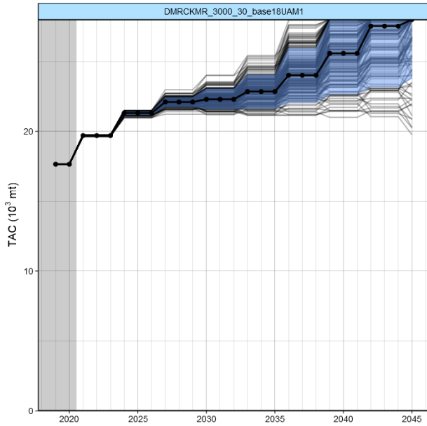
Figure 2b. Worm plots for TAC and TRO (reported as “Relative SSB index”) for DMRCKMR , when tuned to 30% of TRO_0 in the year 2035, for the RC (base18). The blue shadings represent 95% probability envelopes, and the bold line with dots shows the medians. In the TRO plots, the red line is the SSB level corresponding to the interim rebuilding target (0.20 SSB 0 ) of the Extended Commission, and the green band represents the 80% confidence interval for the maximum sustainable yield (MSY), with the median as the horizontal green line. The TAC axis upper bound is at the maximum TAC of 28 000 mt which the CMP allows.
