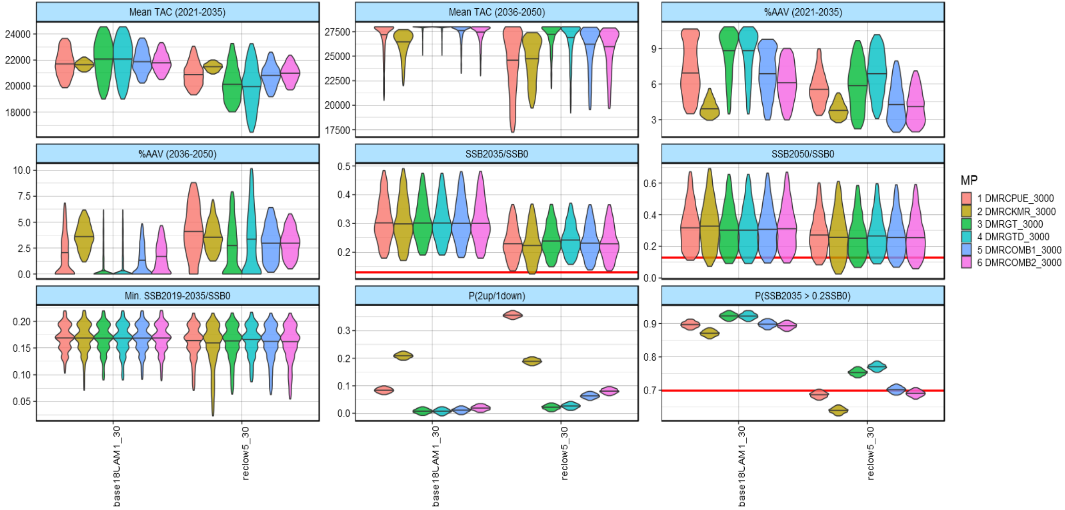
Figure 1. “Guitar plots” of performance statistics for the six CMPs investigated.
