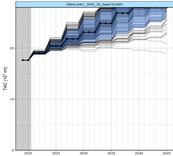
Figure 2e. Worm plots for TAC and TRO (reported as “Relative SSB index”) for DMRCOMB1 , when tuned to 30% of TRO_0 in the year 2035, for the RC (base18). The blue shadings represent 95% probability envelopes, and the bold line with dots shows the medians. In the TRO plots, the red line is the SSB level corresponding to the interim rebuilding target (0.20 SSB_0 ) of the Extended Commission, and the green band represents the 80% confidence interval for the maximum sustainable yield (MSY), with the median as the horizontal green line. The TAC axis upper bound is at the maximum TAC of 28 000 mt which the CMP allows.
