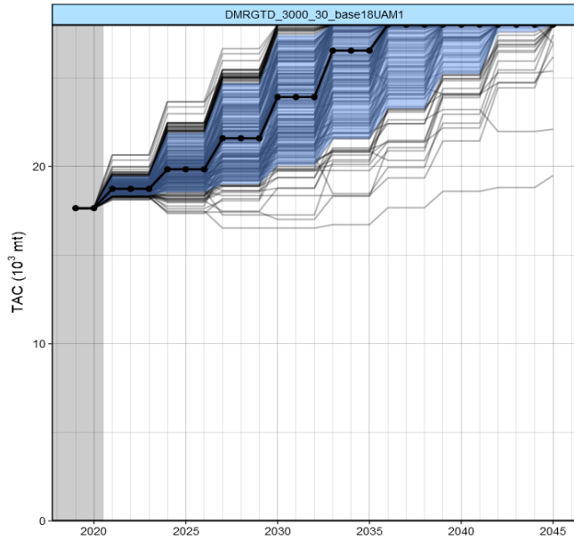
Figure 2d. Worm plots for TAC and TRO (reported as “Relative SSB index”) for DMRGTD , when tuned to 30% of TRO_0 in the year 2035, for the RC (base18). The blue shadings represent 95% probability envelopes, and the bold line with dots shows the medians. In the TRO plots, the red line is the SSB level corresponding to the interim rebuilding target (0.20 SSB0) of the Extended Commission, and the green band represents the 80% confidence interval for the maximum sustainable yield (MSY), with the median as the horizontal green line. The TAC axis upper bound is at the maximum TAC of 28 000 mt which the CMP allows.
