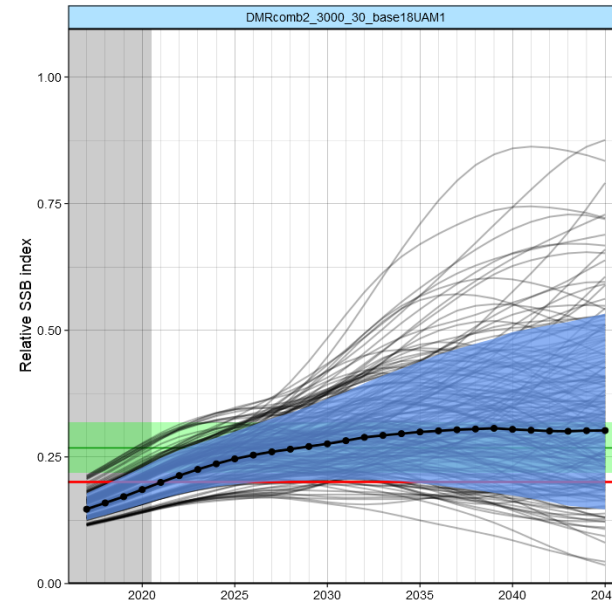
Figure 2f. Worm plots for TAC and TRO (reported as “Relative SSB index”) for DMRCOMB2 , when tuned to 30% of TRO_0 in the year 2035, for the RC (base18). The blue shadings represent 95% probability envelopes, and the bold line with dots shows the medians. In the TRO plots, the red line is the SSB level corresponding to the interim rebuilding target (0.20 SSB 0 ) of the Extended Commission, and the green band represents the 80% confidence interval for the maximum sustainable yield (MSY), with the median as the horizontal green line. The TAC axis upper bound is at the maximum TAC t of 28 000 mt which the CMP allows.
