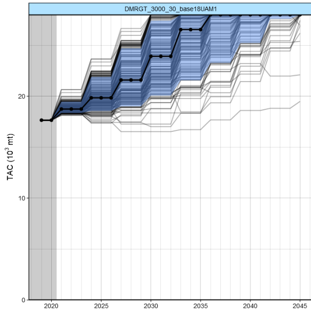
Figure 2c. Worm plots for TAC and TRO (reported as “Relative SSB index”) for DMRGT , when tuned to 30% of TRO_0 in the year 2035, for the RC (base18). The blue shadings represent 95% probability envelopes, and the bold line with dots shows the medians. In the TRO plots, the red line is the SSB level corresponding to the interim rebuilding target (0.20 SSB 0 ) of the Extended Commission, and the green band represents the 80% confidence interval for the maximum sustainable yield (MSY), with the median as the horizontal green line. The TAC axis upper bound is at the maximum TAC of 28 000 mt which the CMP allows.
