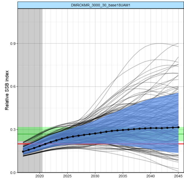
Figure 2b. Worm plots for TAC and TRO (reported as “Relative SSB index”) for DMRCKMR , when tuned to 30% of TRO_0 in the year 2035, for the RC (base18). The blue shadings represent 95% probability envelopes, and the bold line with dots shows the medians. In the TRO plots, the red line is the SSB level corresponding to the interim rebuilding target (0.20 SSB 0 ) of the Extended Commission, and the green band represents the 80% confidence interval for the maximum sustainable yield (MSY), with the median as the horizontal green line. The TAC axis upper bound is at the maximum TAC of 28 000 mt which the CMP allows.
