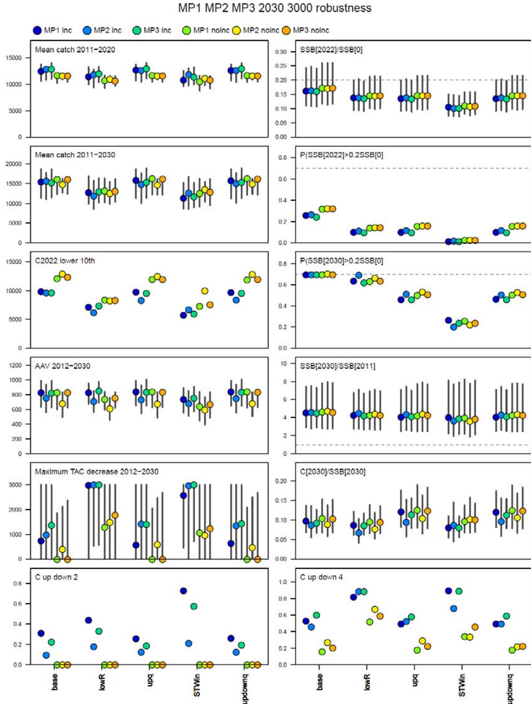
Figure 7. Statistics comparing the performance of MP1 , MP2 and the Bali Procedure (referred to in this figure as MP3) for procedures tuned to 2030 and 3000 t maximum change in TAC, under the base case and four robustness trials (low recruitment, qup=catchability increase, using the ST windows CPUE time series, and qupdown=catchability increase then decrease).
