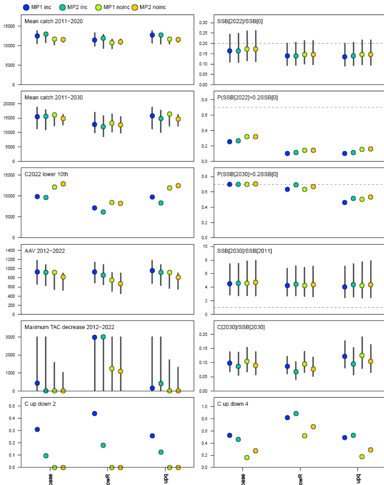
Figure 6. Statistics comparing the performance of MP1 and MP2 for procedures tuned to 2030 and 3000 t maximum change in TAC, allowing either an increase (inc) or no increase (noinc) in 2013. AAV is average annual catch. “C up down 2” is the probability that the TAC goes up and then down in the first two MP decision years (2013, 2016); “C up down 4” is the probability that the TAC goes up then down in any of the first four MP decision years (2013, 2016, 2019, 2022).
