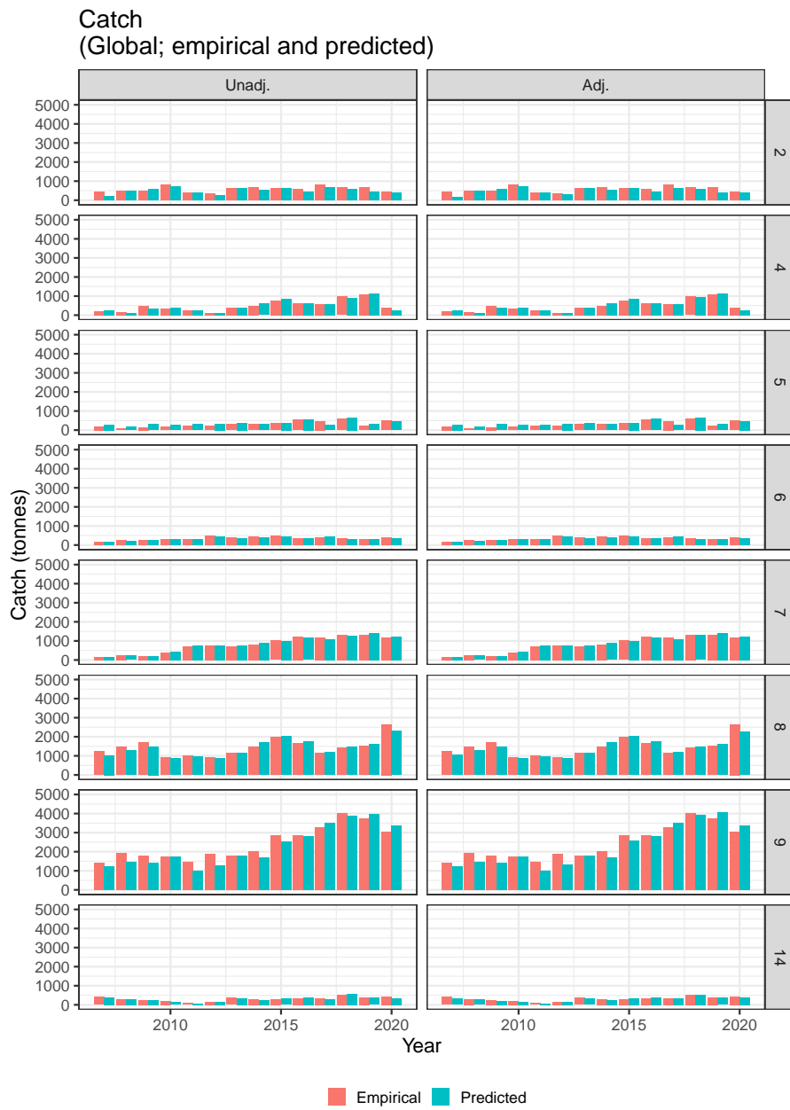
Figure 23: Global prediction of empirical CCSBT catch data, per CCSBT statistical area. Model runs assuming an Uadjusted and Adjusted catch rate are shown.
