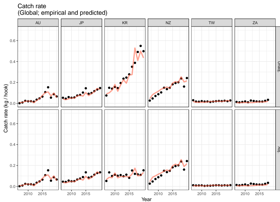
Figure 20: Global model fit to updated (2023) empirical CCSBT catch rate data, per CCSBT member flag. Catch rate is calculated as the mean of the catch over effort. Observed values are shown as points. Model runs assuming an Uadjusted and Adjusted catch rate are shown.
