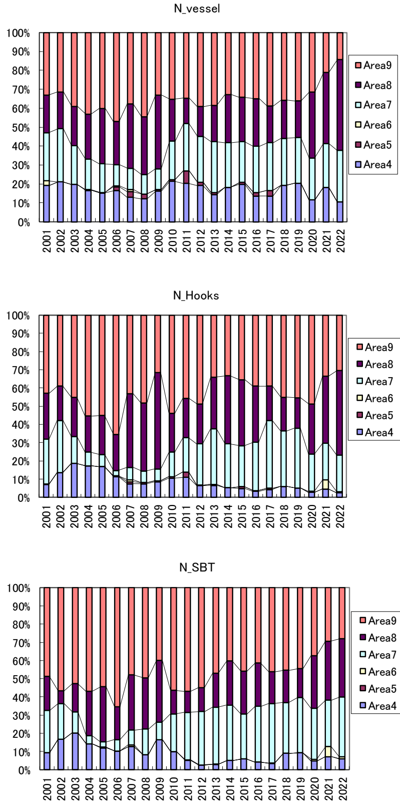
Fig. 2. Proportions of Area in the number of vessels, the number of hooks used and the number of SBT caught in 2022 and previous years in RTMP data.
