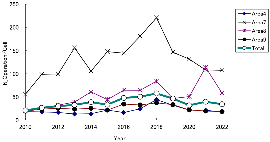
Fig. 9. Changes of the number of longline operations per cell (5 degrees latitude and longitude and month) over 13 years in Area 4-9 in RTMP data.
