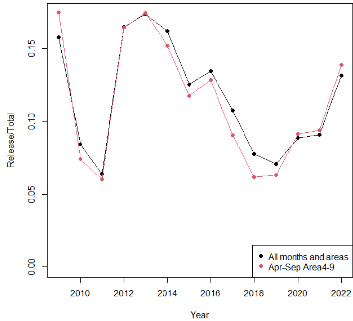
Fig. 6. Proportion of SBT released/discarded in total catch (retained + released + discarded) by year.
