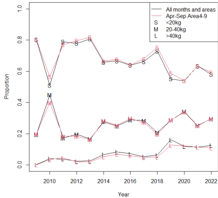
Fig. 7. Proportion of SBT released/discarded in three body weight categories against the total number of released/discarded fish of the year.
