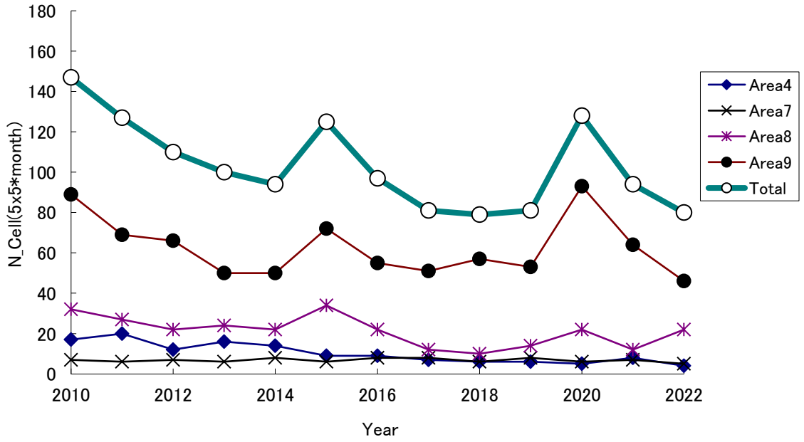
Fig. 8. Changes of the number of cells (5 degrees latitude and longitude and month) operated over 13 years in Area 4-9 in RTMP data.
