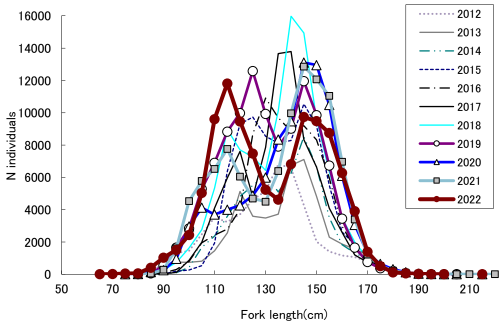
Fig. 3. Length frequency distributions of SBT by year in 2022 and previous 10 years in RTMP data.
