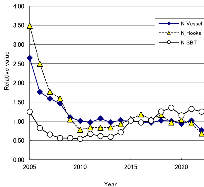
Fig. 1. Number of operation, number of vessels and number of SBT caught in Area 4-9 in 2022 and previous years in RTMP data.
