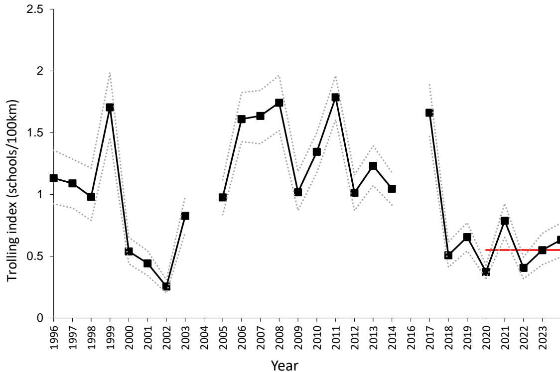
Figure 2. Grid-type trolling index, showing number of schools per 100 km off the Western Australian coast in January. Dashed lines are 90% confidence intervals. The red line shows the average 5-year median value.
