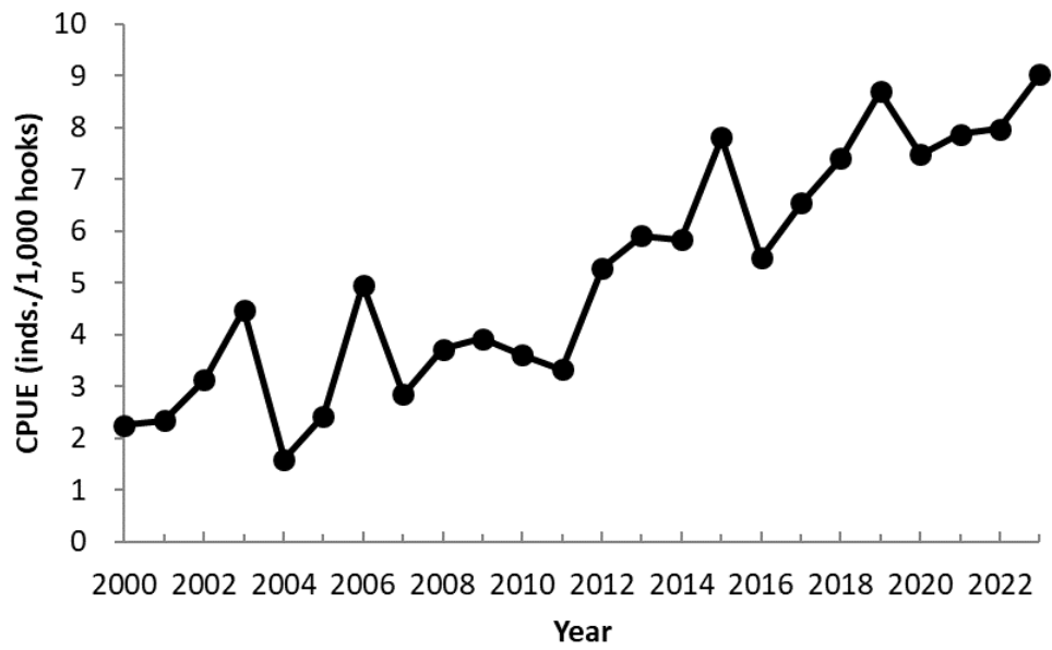
Fig. 2. The nominal CPUE series of Korean tuna longline vessels targeting SBT during 2000-2023.
