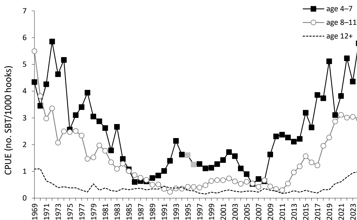
Figure 11 Nominal CPUE of ages 4–7, 8–11 and 12+ SBT for Japanese longliners operating in statistical areas 4–9 in months 4–9.
