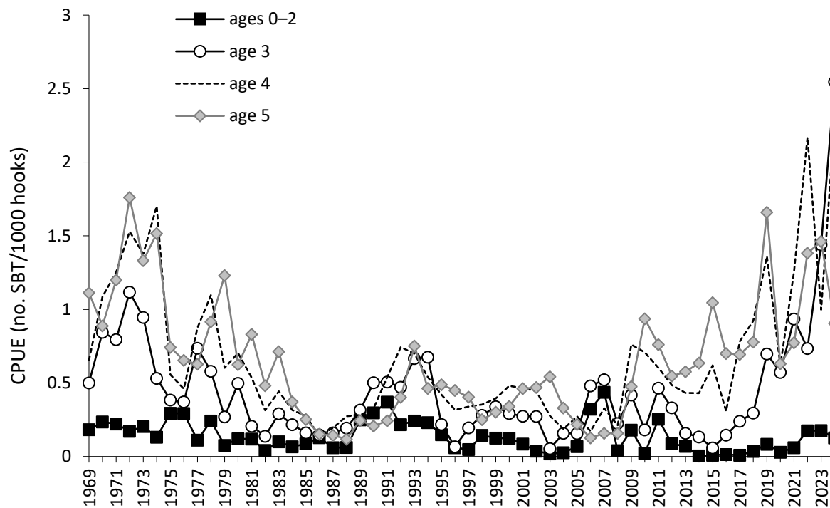
Figure 12 Nominal CPUE of ages 0–2, 3, 4 and 5 SBT for Japanese longliners operating in statistical areas 4–9 in months 4–9.
