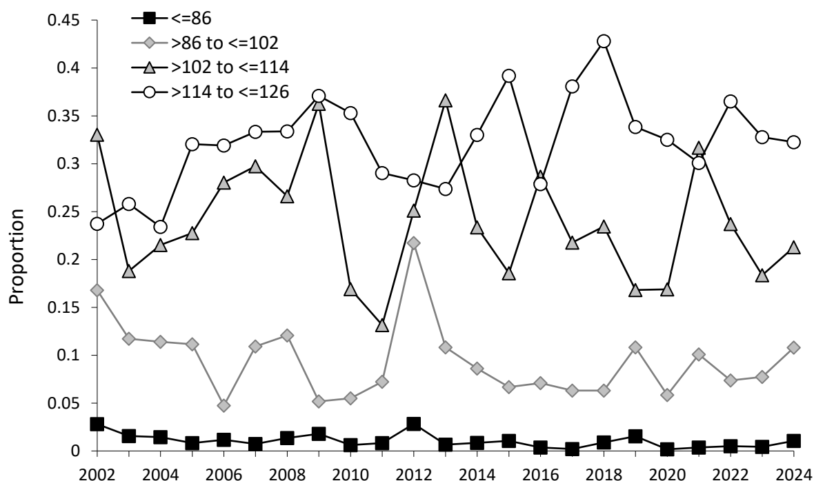
Figure 20 Size composition (proportion of total catch) of juvenile SBT caught by Taiwanese longliners
