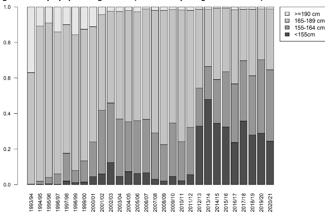
Figure 7 Size composition of SBT caught on the spawning grounds by the Indonesian longline fishery by spawning season (from Sulistyaningsih et al. 2020).
