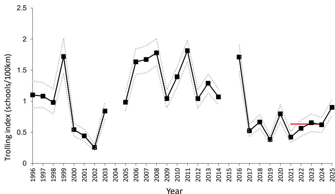
Figure 2 Grid-type trolling index, showing number of schools per 100 km off the Western Australian coast in January. Dashed lines are 90% confidence intervals. The red line shows the average 5-year median value.
