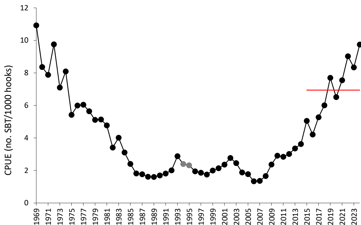
Figure 10 Nominal CPUE of age 4+ SBT for Japanese longliners operating in statistical areas 4–9 in months 4–9. The horizontal line is the 10-year mean.
