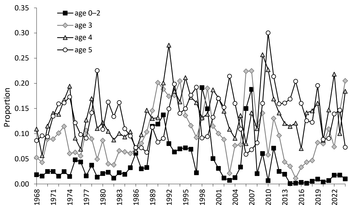
Figure 18 Age composition (proportion of total catch) of ages 0–2, 3, 4 and 5 in the Japanese longline fishery in statistical areas 4–9, months 4–9
