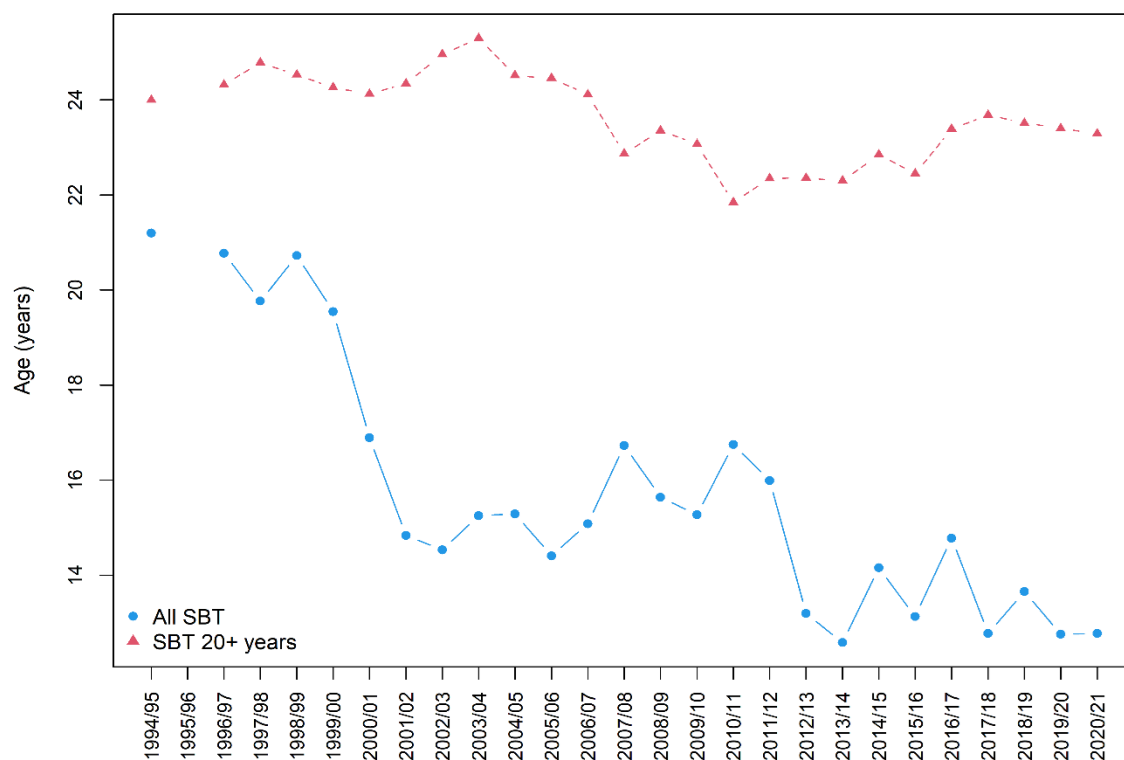
Figure 8 Mean estimated age (years) of SBT caught on the spawning grounds by Indonesian longliners (from Sulistyaningsih et al. 2020).
