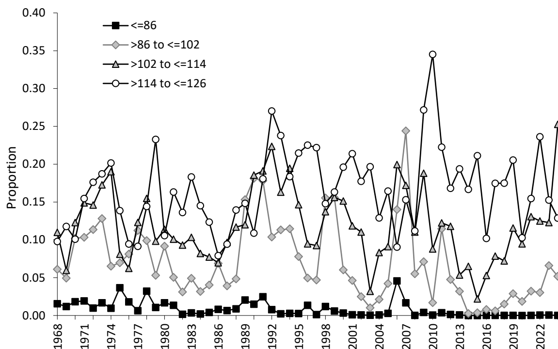
Figure 19 Size composition (proportion of total catch) of juvenile SBT caught by Japanese longliners in statistical areas 4–9, months 4–9
