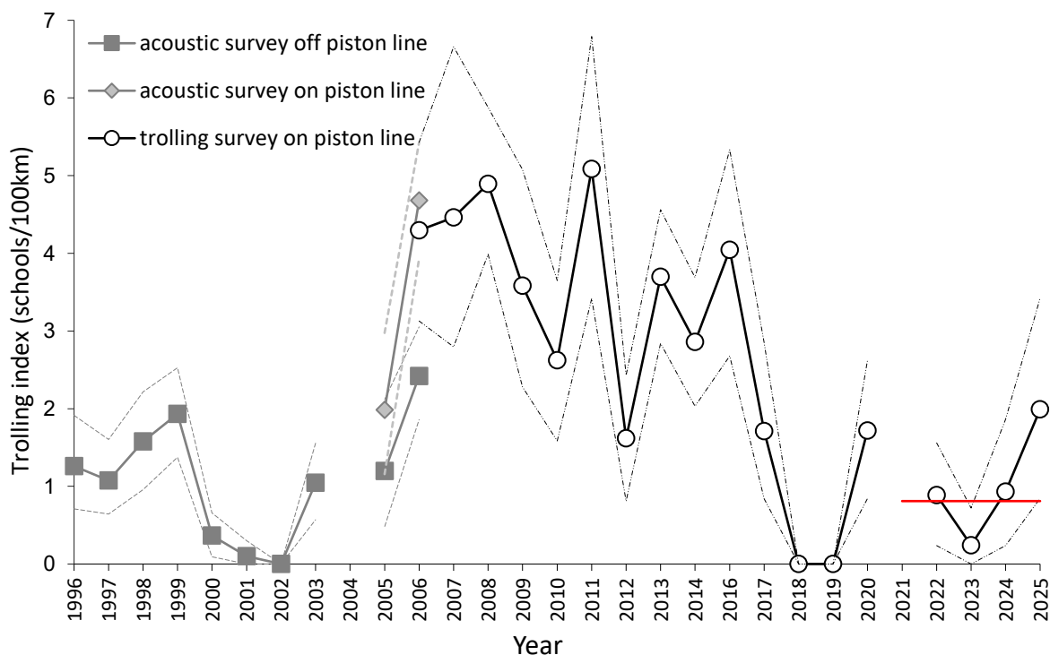
Figure 1 Trolling index, showing number of schools per 100 km off the Western Australian coast in January. Dashed lines are 90% confidence intervals. The red line shows the average 5-year median value.
