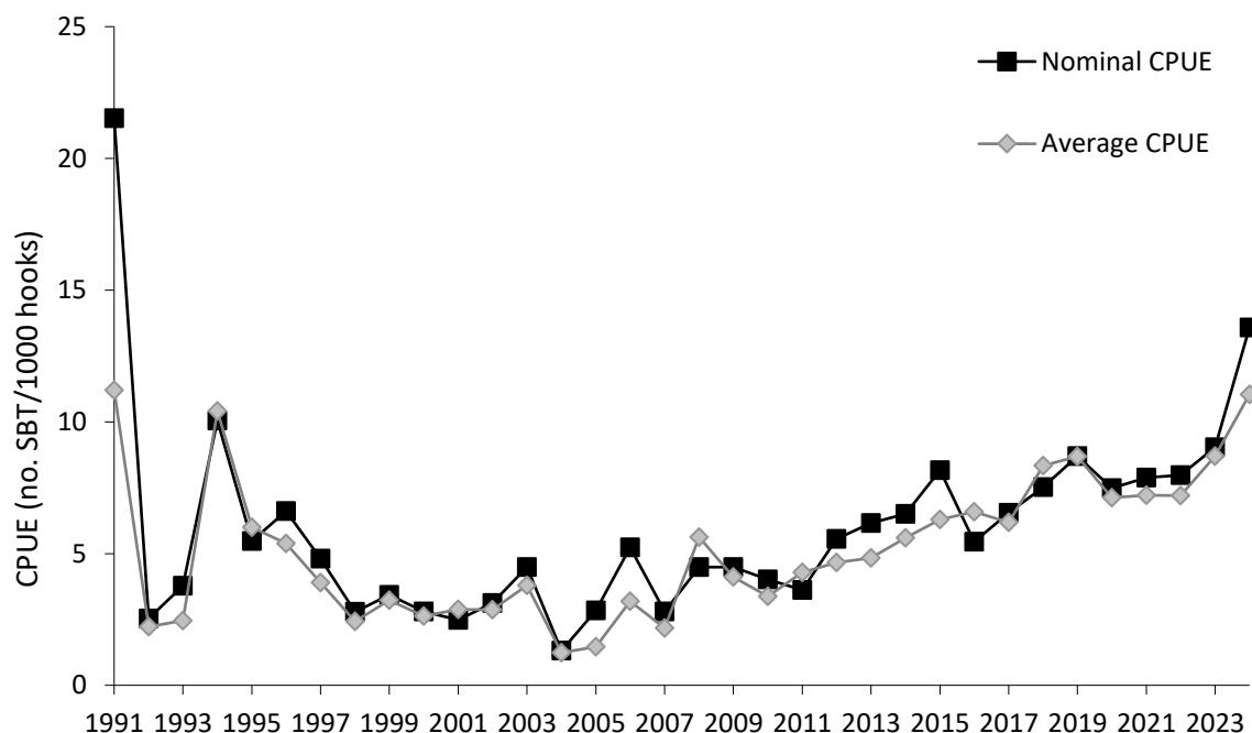
Figure 14 Nominal and average CPUE of total SBT for Korean longliners operating in statistical areas 4–9 in months 4–9.
