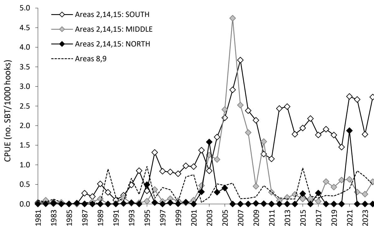
Figure 16 Nominal CPUE of SBT for Taiwanese longliners operating in statistical areas 2, 14 and 15 (pooled) by 5° latitudinal strips in months 4–9
