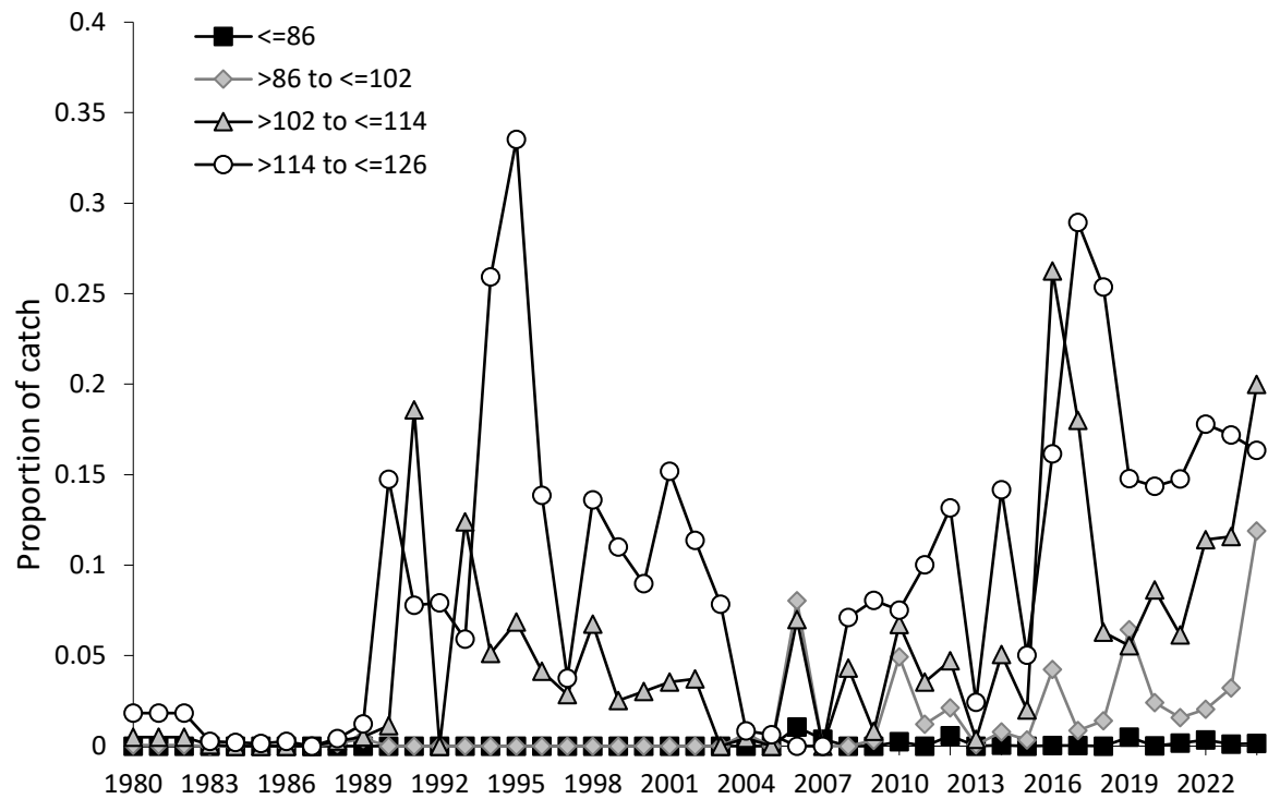
Figure 5 Size composition of juvenile fish (< 6 years) for the NZ domestic longline fishery
