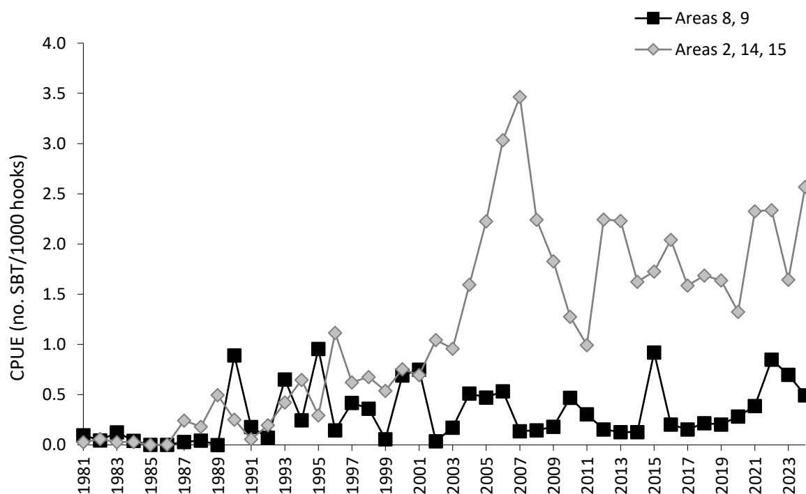
Figure 15 Nominal CPUE of SBT for Taiwanese longliners operating in statistical areas 8 and 9 (pooled) and 2, 14 and 15 (pooled) in months 4–9
