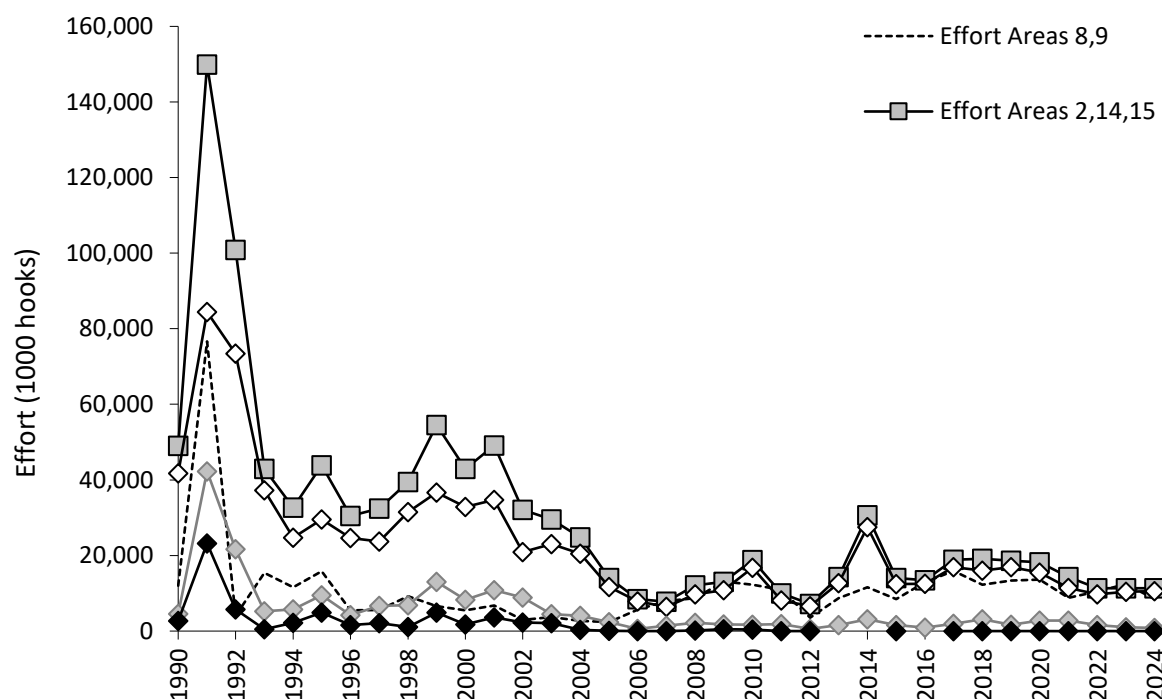
Figure 17 Effort (1000 hooks) from Taiwanese longliners in statistical areas 8 & 9 (pooled) and 2, 14 and 15 (pooled). Areas 2, 14 and 15 are also separated into 5° latitudinal strips for months 4–9.
