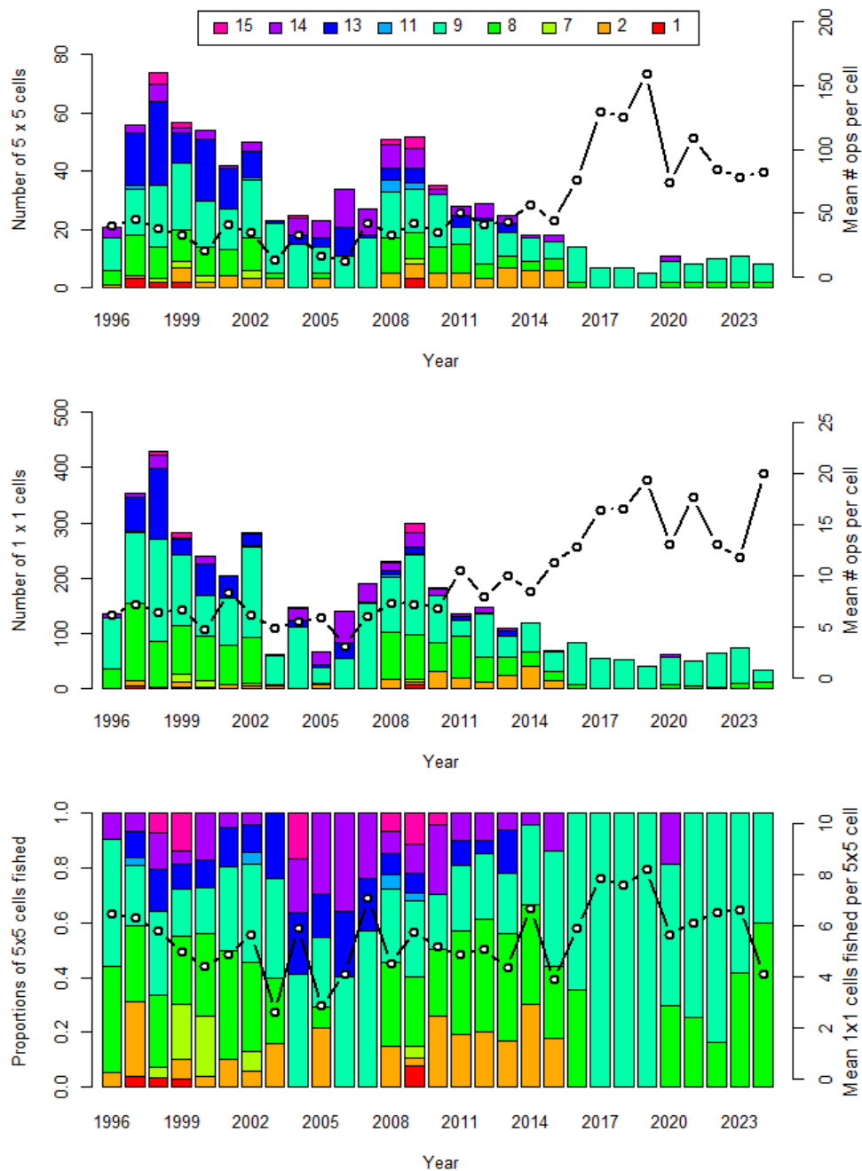
Fig. 9. (Upper) Bars represent the number of major cells (5°x5° by month) fished by CCSBT statistical area and year, see left y-axis. The line represents the mean annual operations per cell, see right y-axis. (Middle) As for upper plot, but with minor cells (1x1° by month) instead of major cells. (Lower) Relative distribution of fished major cells by the proportion of the cell fished, measured as the number of minor cells fished within each major cell, see left y-axis. The lowest (red) and highest (purple) bands represent major cells in which, respectively, 1 and 15 of the 25 minor cells were fished. The line represents the mean number of minor cells fished per major cell by year, see right y-axis.
