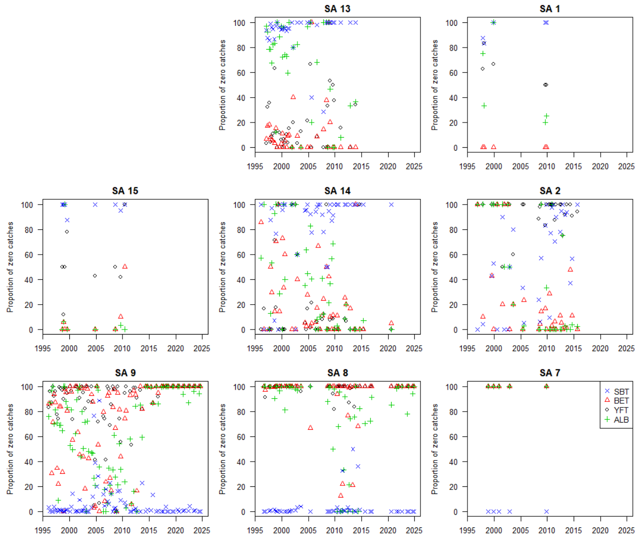
Fig. 6. Proportion of zero catches per set by year-quarter, species, and statistical area, for yellowfin, bigeye, albacore, and southern bluefin tuna.
