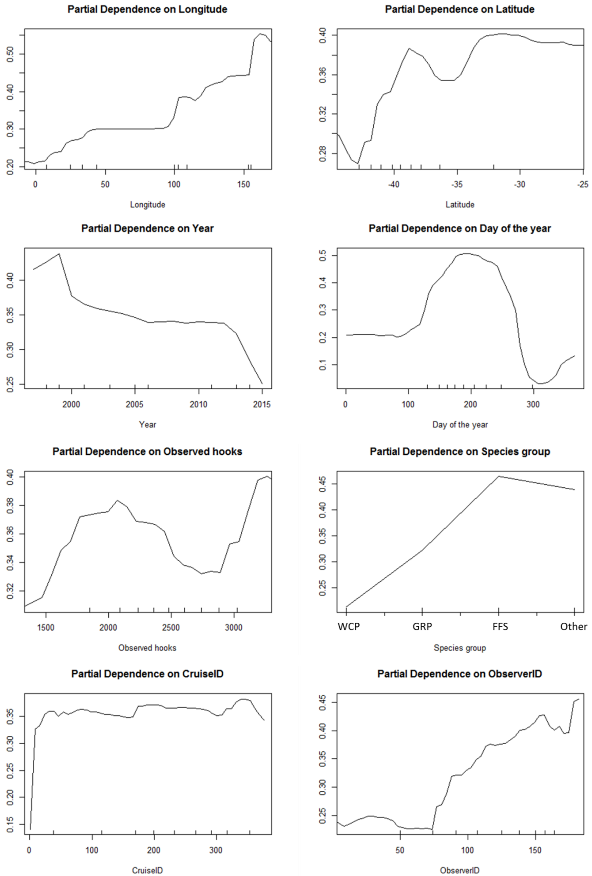
Fig. 5 Petrel model. Figures show that the partial dependences associated with changes of each variation. The Y axis indicates the partial dependence. The larger value means lower probabilities of bycatch.
