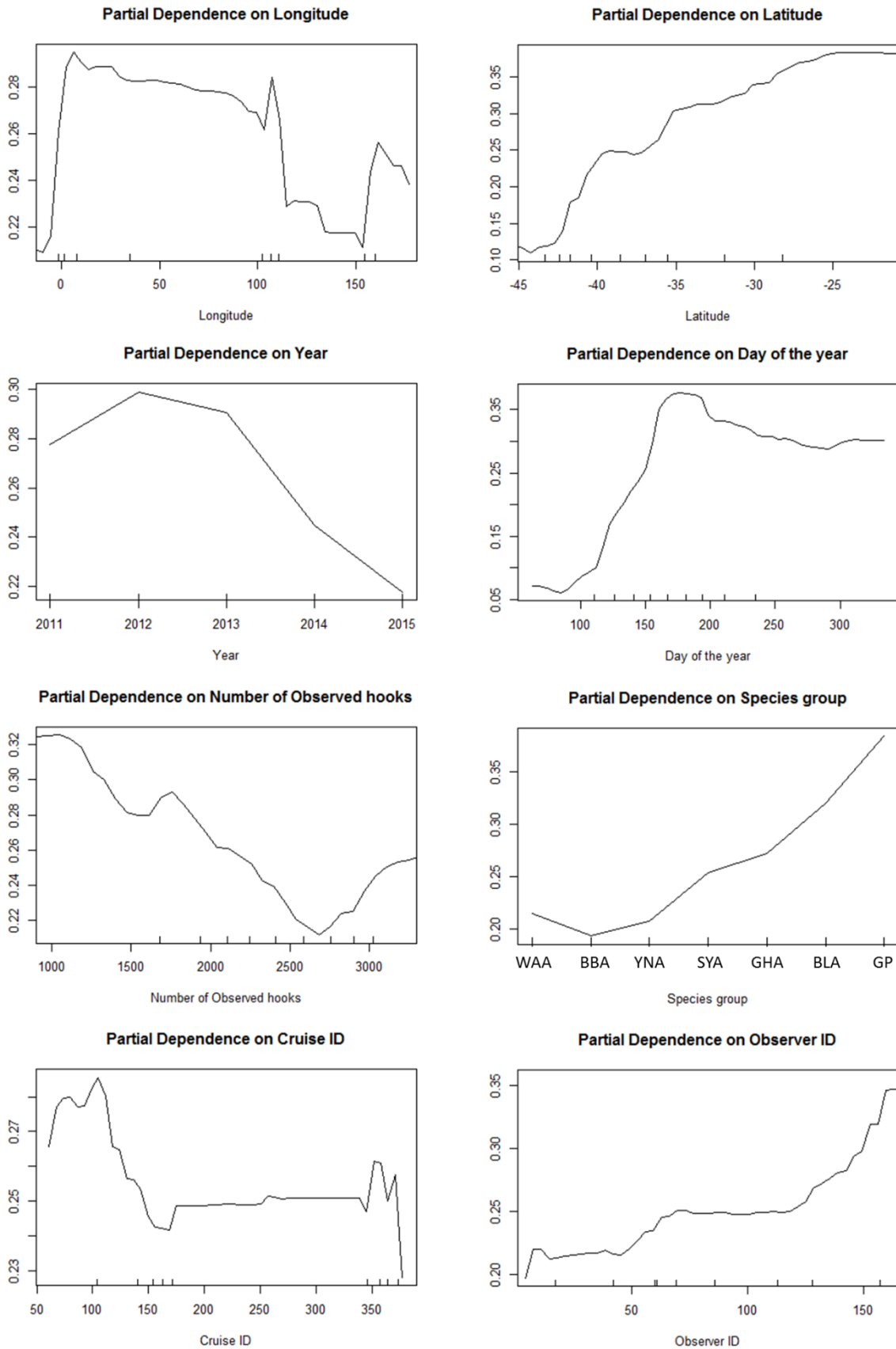
Fig. 4 Albatross mitigation model. Figures show that the partial dependences associated with changes of each variation. The Y axis indicates the partial dependence. The larger value means lower probabilities of bycatch.
