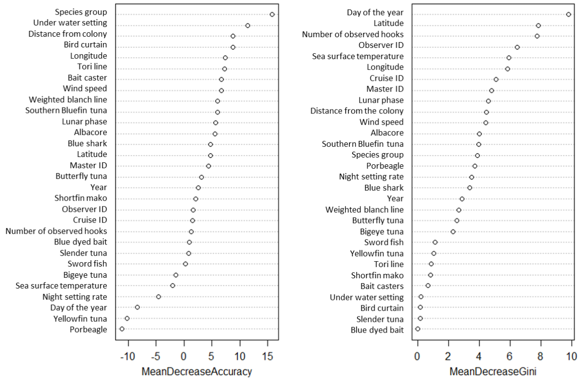
Fig. 2-d Petrel mitigation model
