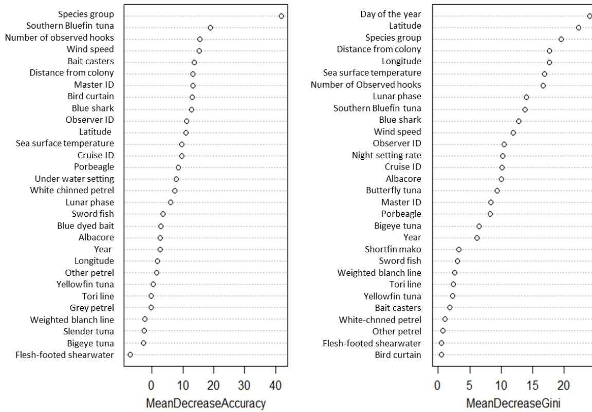
Fig. 2-b Albatross mitigation model
