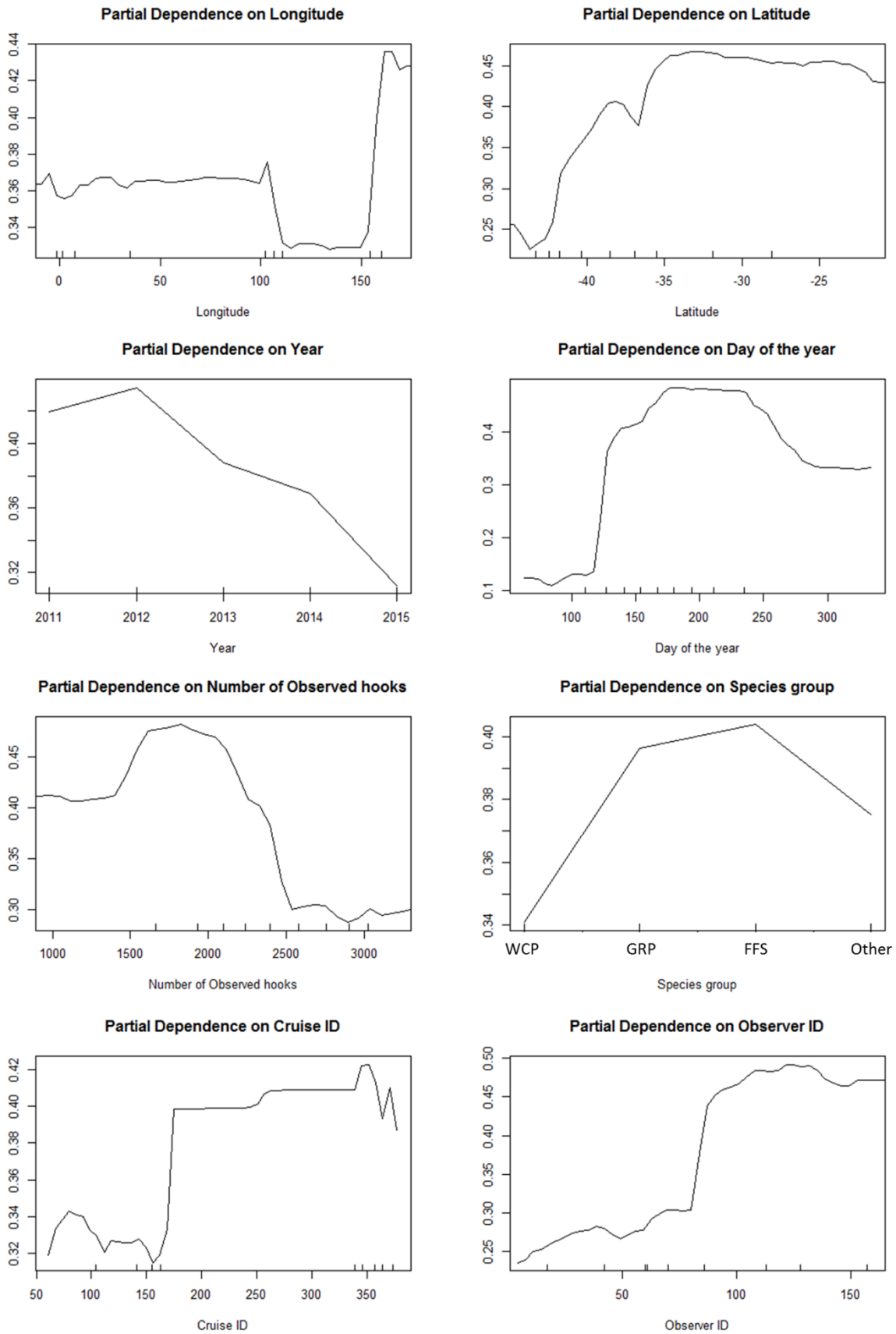
Fig. 6 Petrel mitigation model. Figures show that the partial dependences associated with changes of each variation. The Y axis indicates the partial dependence. The larger value means lower probabilities of bycatch.
