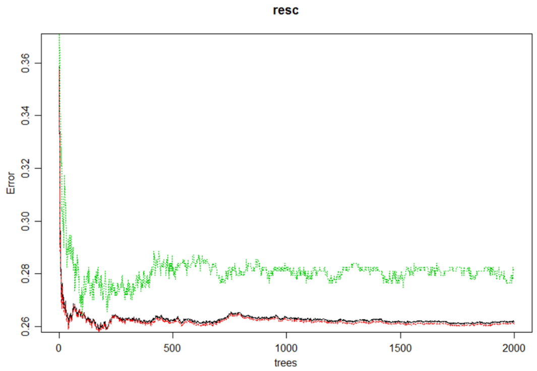
Fig. 1-b Albatross mitigation measure model
