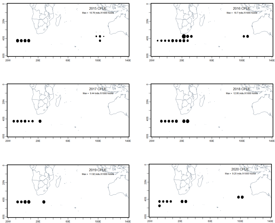
Fig. 1. The distributions of nominal SBT CPUE of Korean longline fisheries, 2015-2020.
