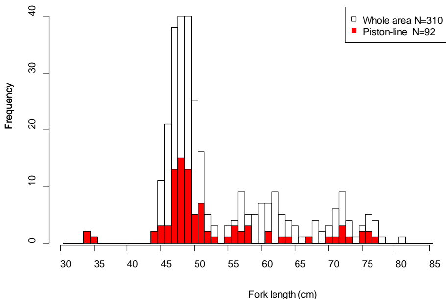
Figure 3 Fork length frequency distributions of southern bluefin tuna caught in the 2016 cruise. That of fish caught off Bremer Bay (119E-120E) is also show as Piston-line.
