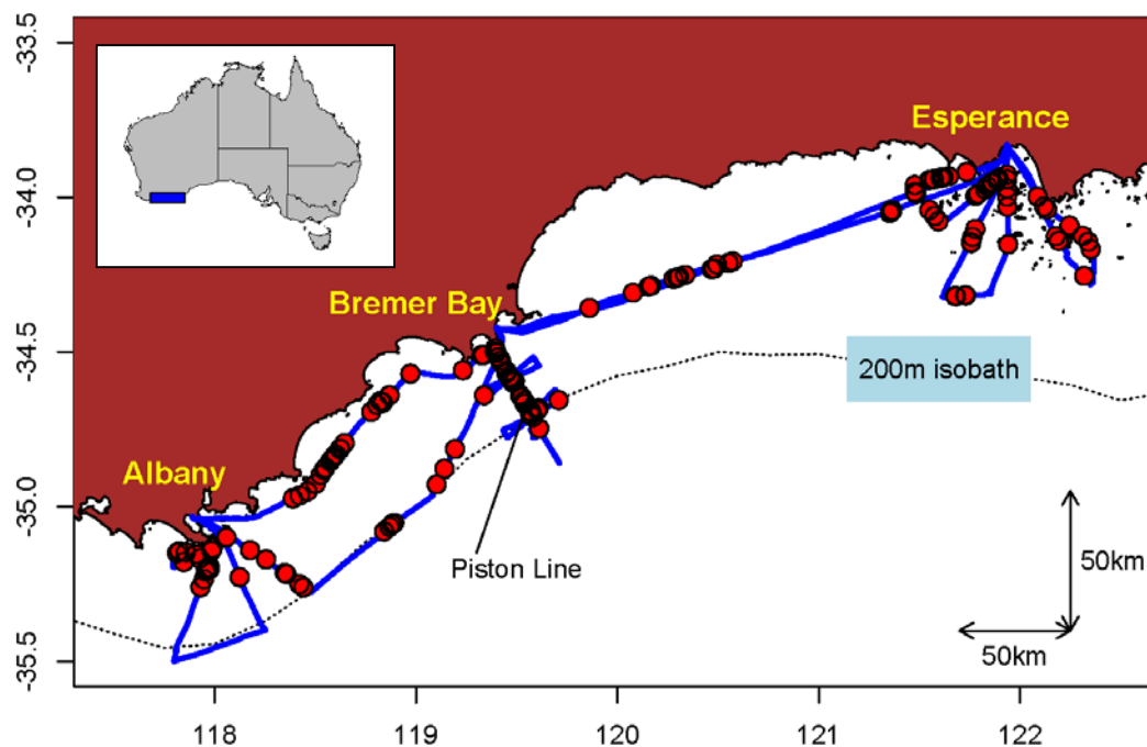
Figure 2 Trajectory of the vessel and location of SBT caught (circles) in the 2016 trolling survey.
