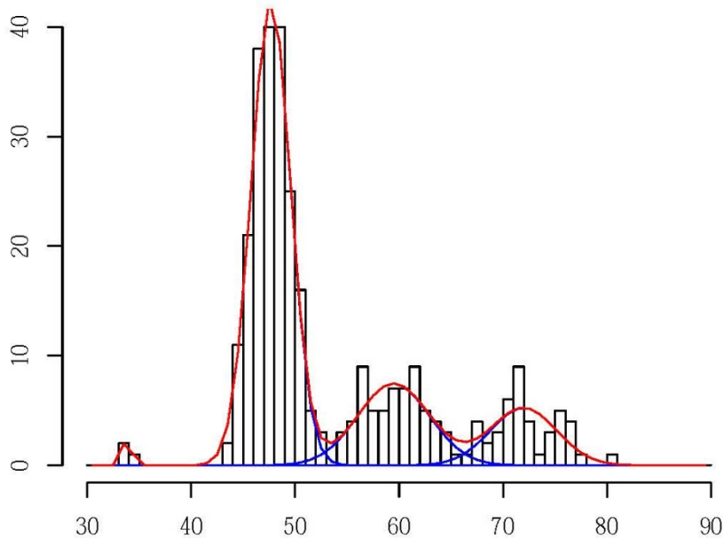
Figure 4 Applied mixed normal distribution to the length frequency distribution of SBT caught in 2016 survey.
