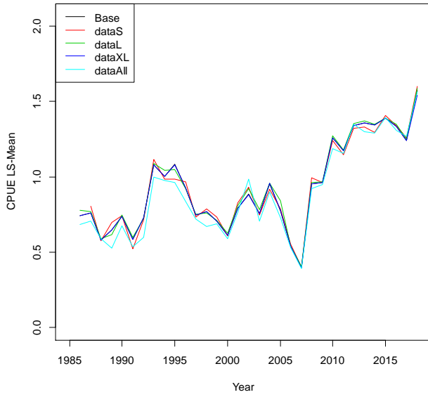
Fig. 8. Sensitivity test of ls-mean of CPUE in various datasets.
