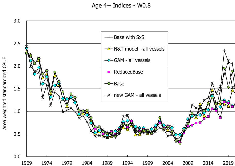
Fig. 1-6. Trends of various abundance indices for age 4+: Base model (Base) with core vessels data (Core); Reduced Base model with Core; Base with shot-by-shot Core; Nishida & Tsuji model with all vessels data; GAM with all vessel data; new GAM series with all vessels data prepared for the new series.
