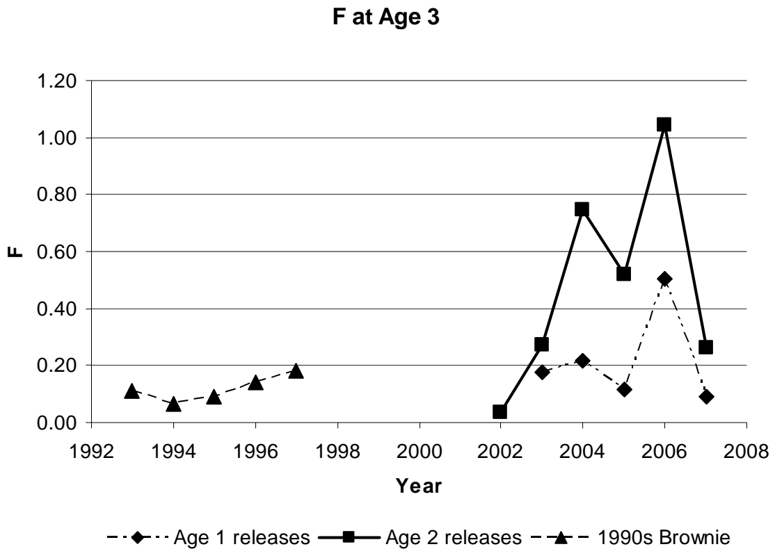
Figure 1: Comparison of fishing mortality rate (F) estimates at ages 3 and 4 obtained from the SRP tagging with those obtained from the 1990s RMP tagging. Estimates for the 1990s tagging were obtained using a Brownie model that integrates data from all release ages.
